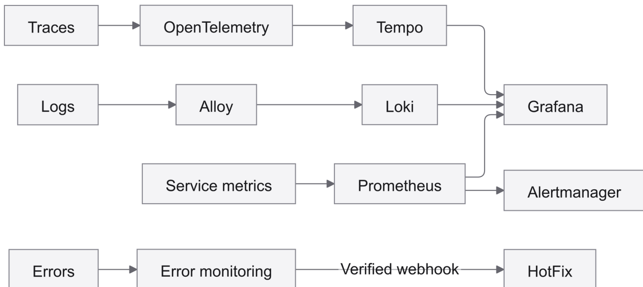
Figure 7. Three signal types, one Grafana. The only path out of the observability stack is the error-monitoring webhook into HotFix.
