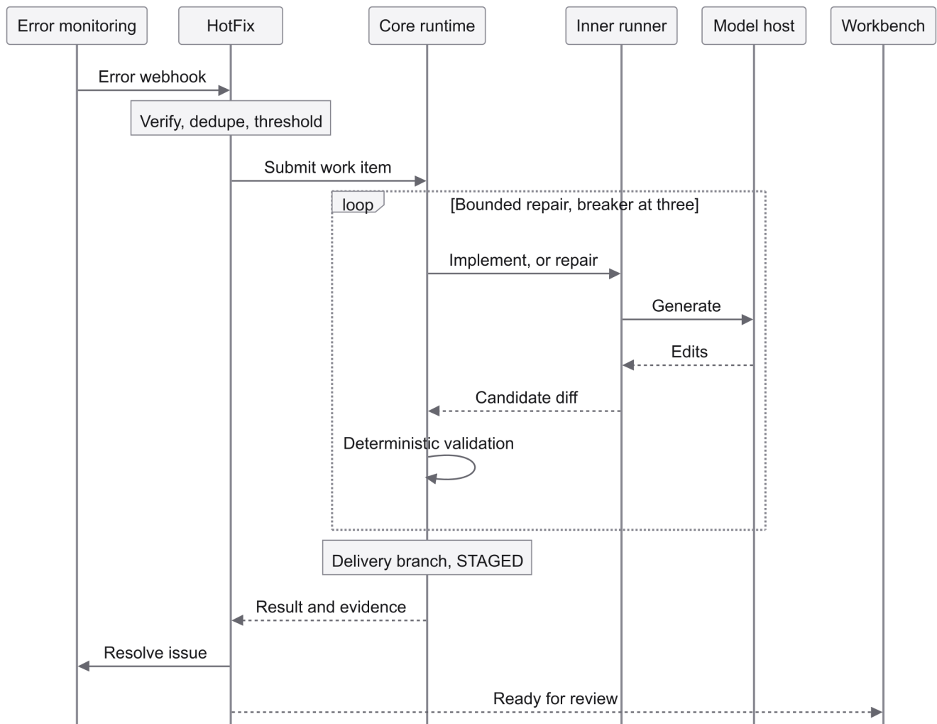
Figure 4. HotFix never takes the model's word: every candidate diff passes deterministic validation inside the loop, the branch stays STAGED until you push, and the linked error issue closes only when the run completes. Platform self-repair follows Figure 6 instead.
